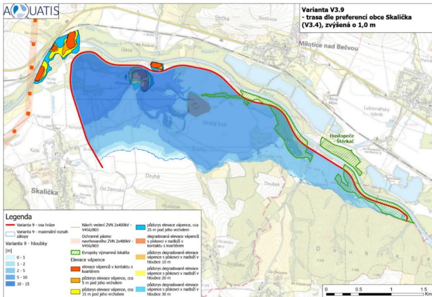
Obr. 11 Situace varianty V3.9 [14]
