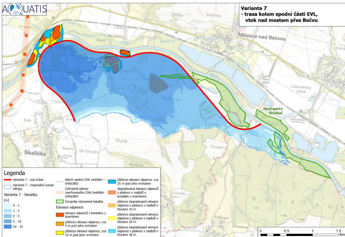
Obr. 9 Situace varianty V3.7 [14]
