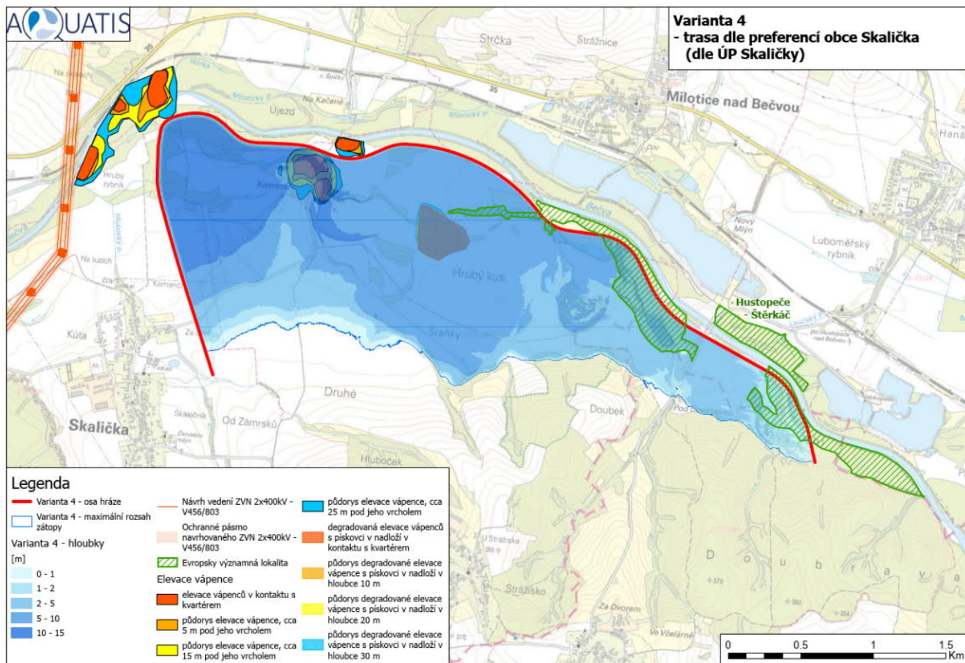
Obr. 6 Situace varianty V3.4 [14]
